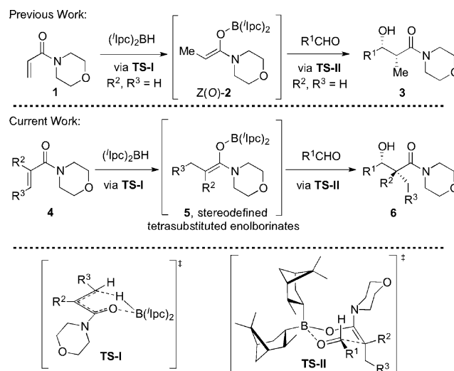
Scheme 1. 1,4-Reductive aldol reactions of substituted \alpha,\beta -unsaturated amides with ( i lpc) 2 BH.
